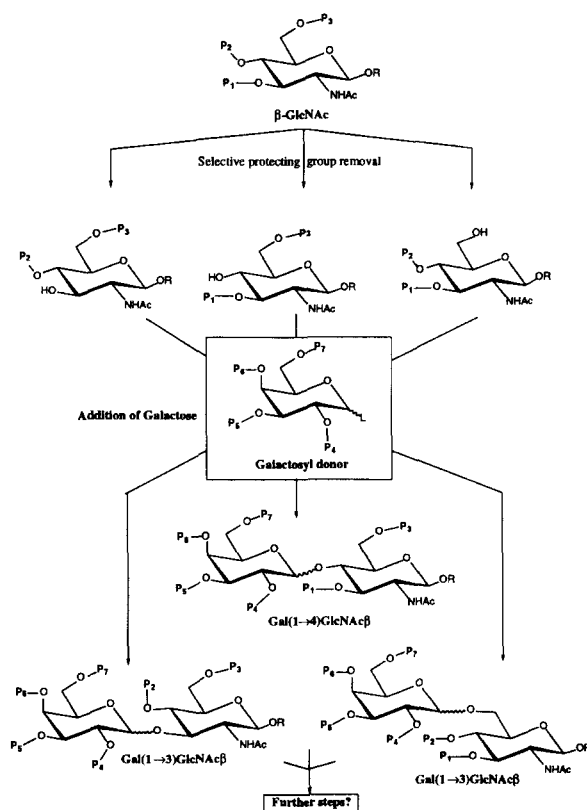
Figure 1. A hypothetical sequence using orthogonally protected monosaccharide building blocks in the process of assembling an oligosaccharide library. Protecting groups P 1 –P 7 must be removable independently.
