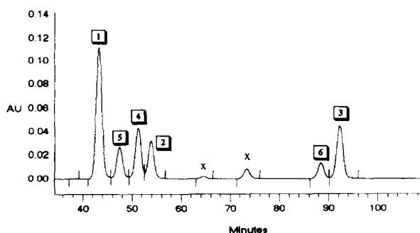
Figure 3. HPLC separation of disaccharides 1–6 produced by random glycosylation of 9 using 30 , as described in Figure 2 and Table 1, entry 5. The elution order of the disaccharides was established by co-injection of synthetic reference standards. 'X' denoted non-carbohydrate UV (292 nm) absorbing contaminants.
