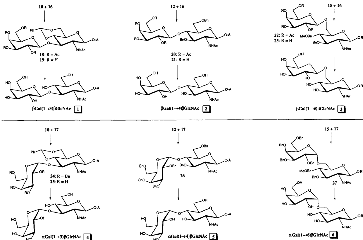
Scheme 2.
